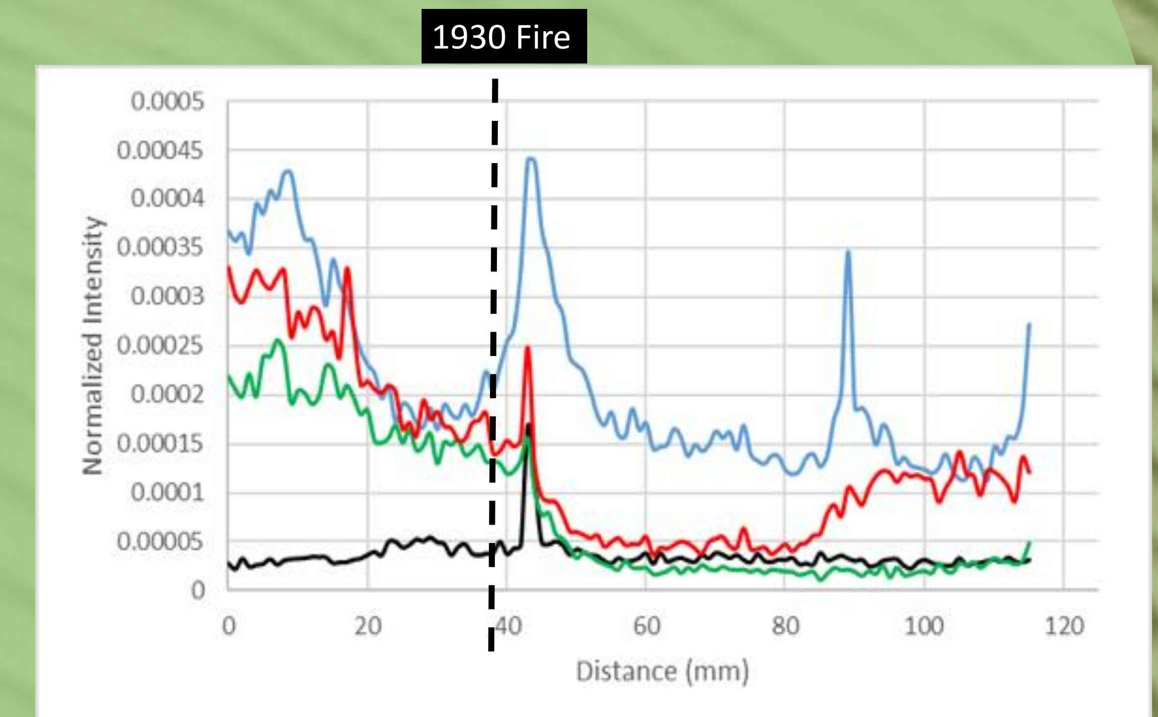
Figure 2: Line graphs of amounts of various elements in a burned Douglas fir tree
